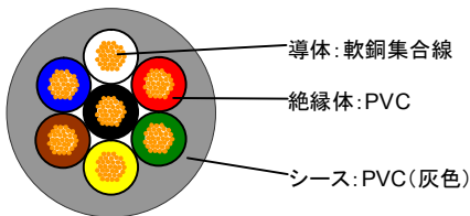
例: VCTF 12 7×0.75mm 2
